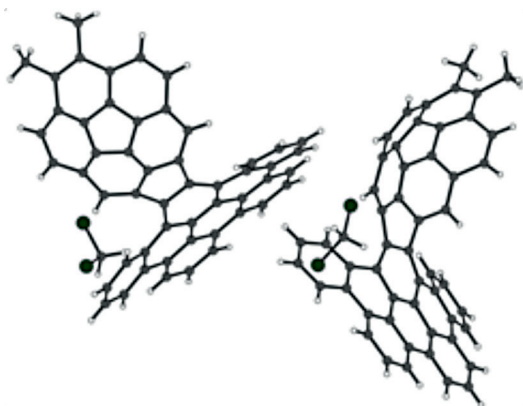
Figure 2. The asymmetric unit in the crystal structure of buckybowl-graphene hybrid 2-Me + 2\cdot\text{CH}_2\text{Cl}_2 .
