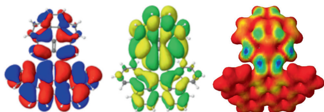
Figure 4. B97D/Def2-TZVPP calculated HOMO (left), LUMO (middle), and nucleophilic LUMO map (right; blue shows highest probability of attack by a nucleophile) of the major conformation of 2\text{-H} .
